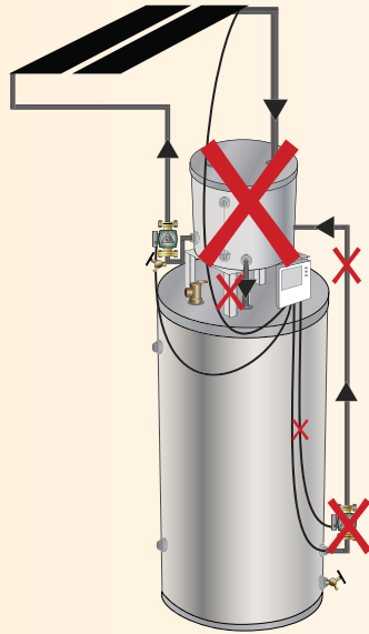
Traditional Drainback
