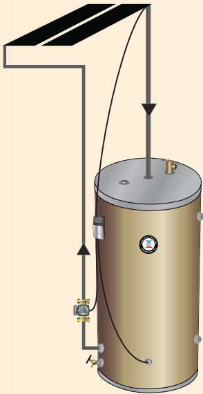
Simple Drainback
